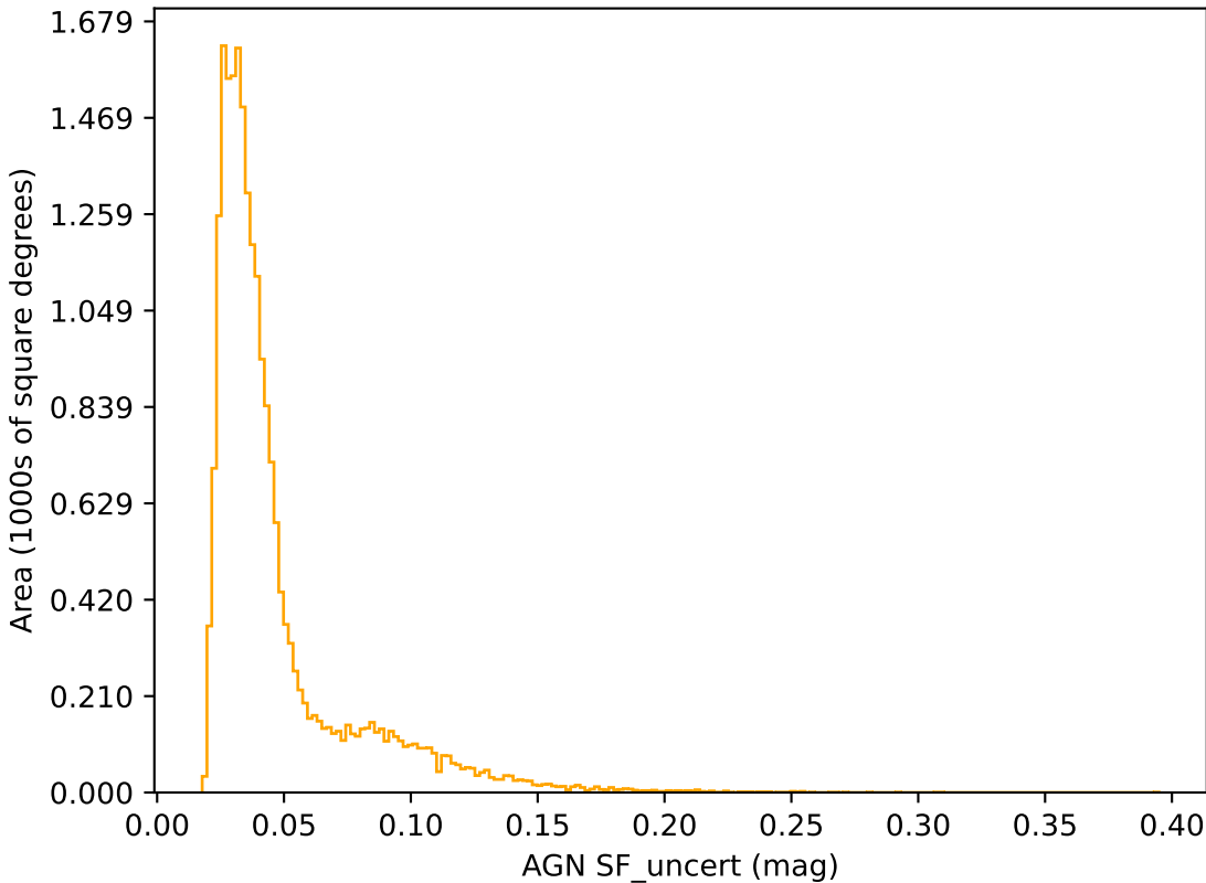
roll_mid2_const_season_v3.3_10yrs r band: AGN SF_uncert
