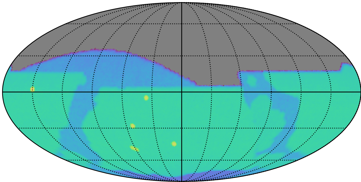
roll_mid2_const_season6v3.3_10yrs z: SurfaceBrightLimit
