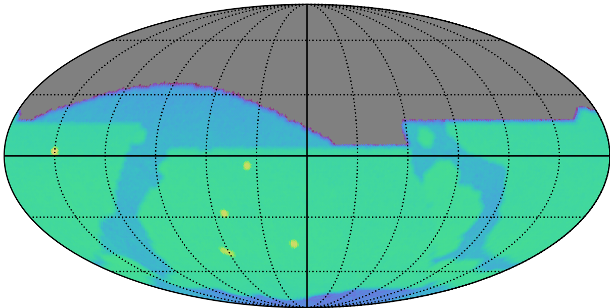
roll_mid2_const_season6v3.3_10yrs r: SurfaceBrightLimit
