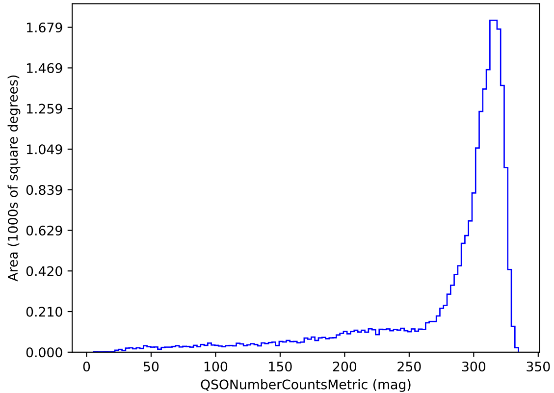
roll_mid2_const_season6v3.3_10yrs u band and non-DD: QSONumberCountsMetric
