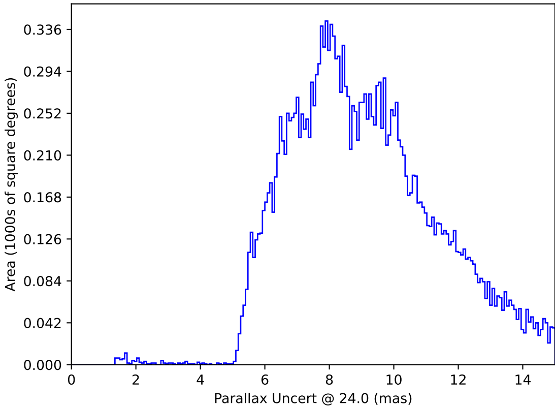
roll_mid2_const_season6v3.3_10yrs : Parallax Uncert @ 24.0
