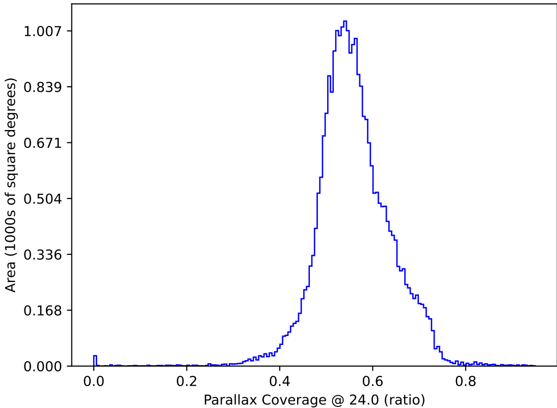
roll_mid2_const_season6v3.3_10yrs : Parallax Coverage @ 24.0
