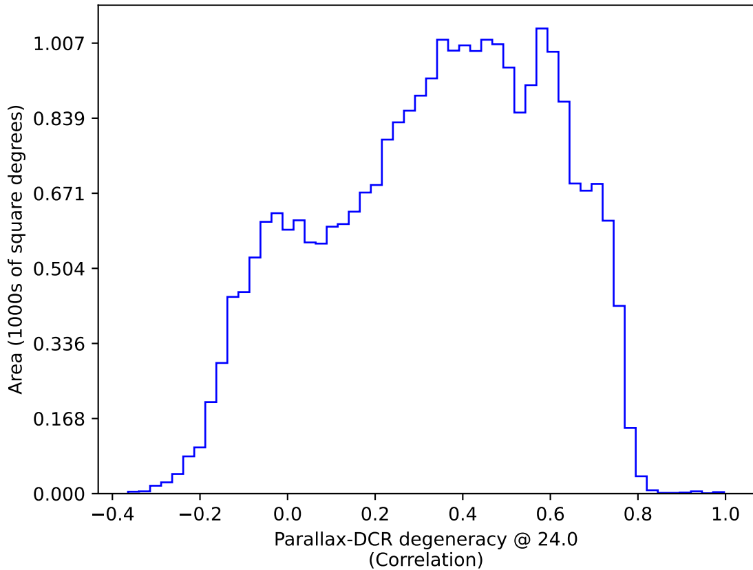
roll_mid2_const_season6v3.3_10yrs : Parallax-DCR degeneracy @ 24.0
