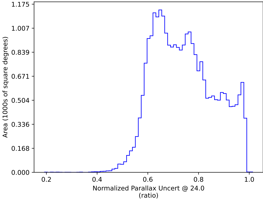
roll_mid2_const_season6v3.3_10yrs : Normalized Parallax Uncert @ 24.0
