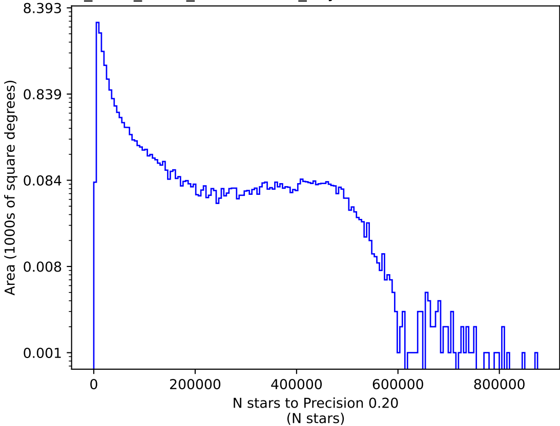
roll_mid2_const_season6v3.3_10yrs i: N stars to Precision 0.20
