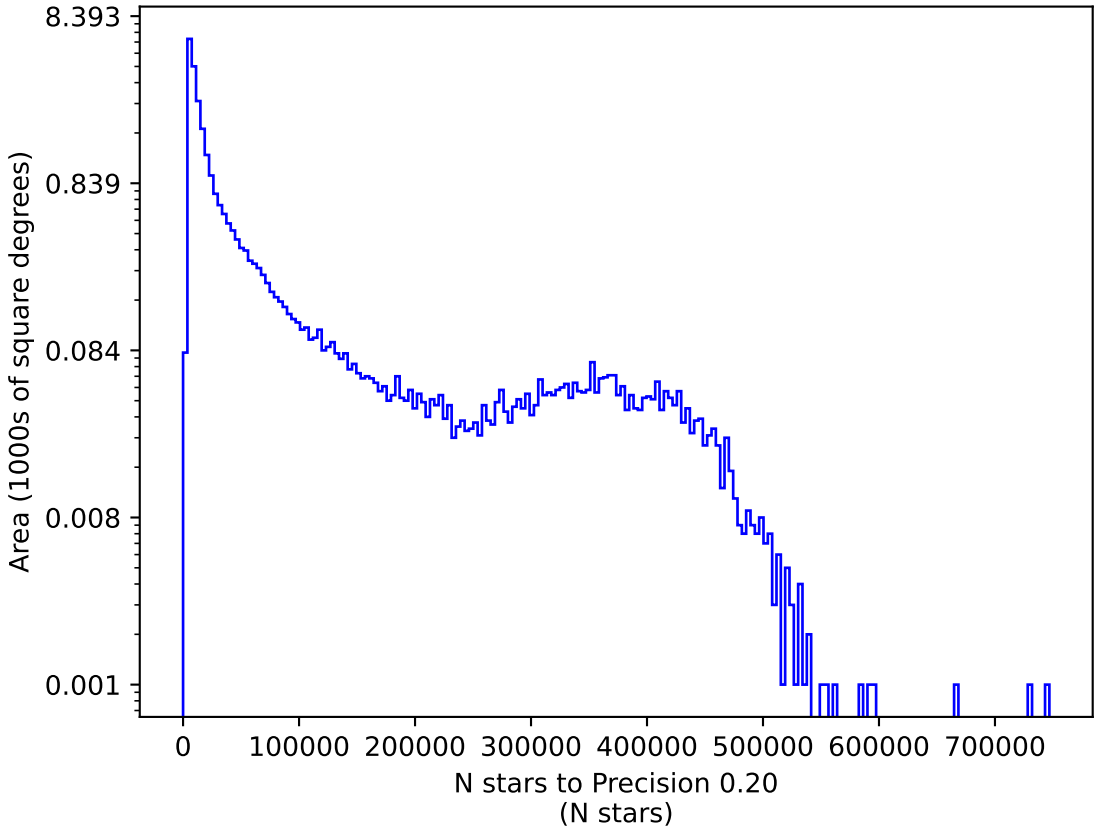
roll_mid2_const_season6v3.3_10yrs g: N stars to Precision 0.20
