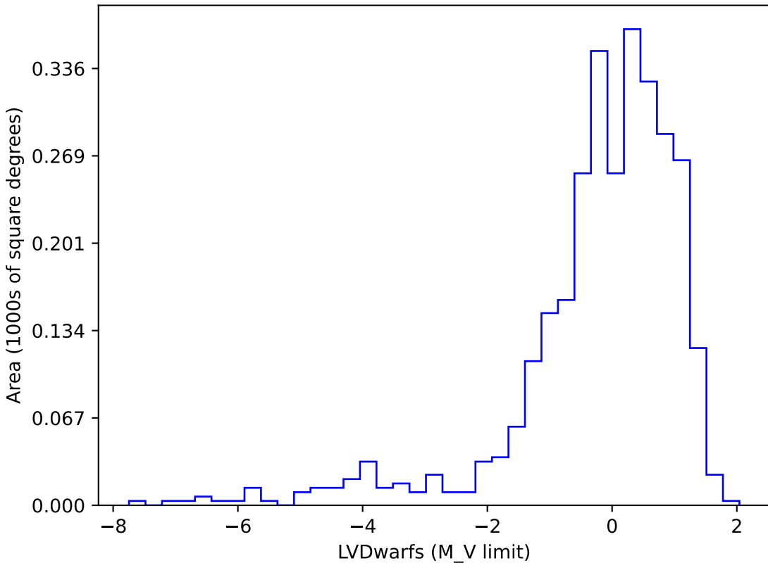
roll_mid2_const_season6v3.3_10yrs gi SCP: LVDwarfs
