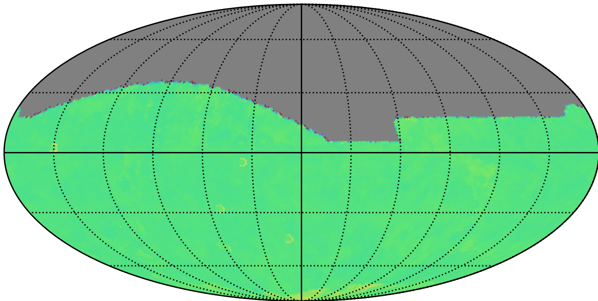
roll_mid2_const_season6v3.3_10yrs r: Kuiper rotTelPos
