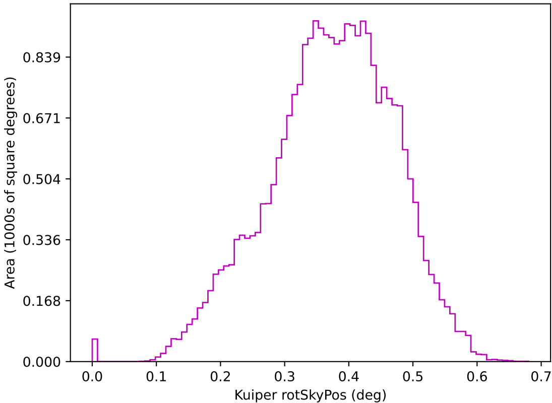
roll_mid2_const_season6v3.3_10yrs z: Kuiper rotSkyPos
