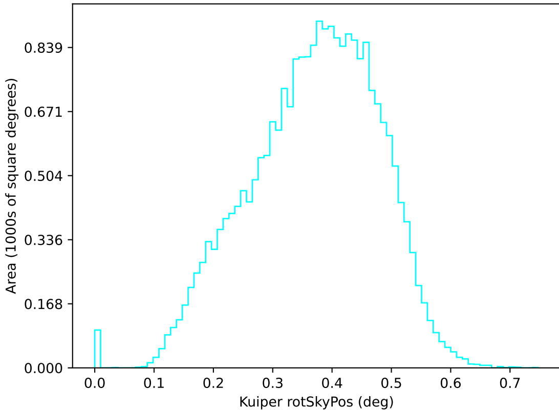
roll_mid2_const_season6v3.3_10yrs u: Kuiper rotSkyPos
