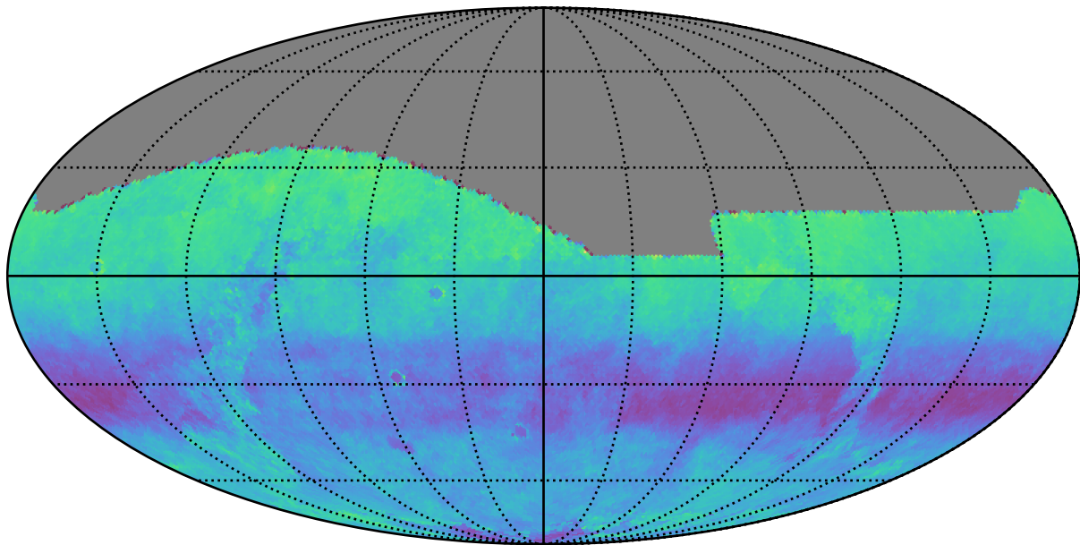
roll_mid2_const_season6v3.3_10yrs r: Kuiper rotSkyPos
