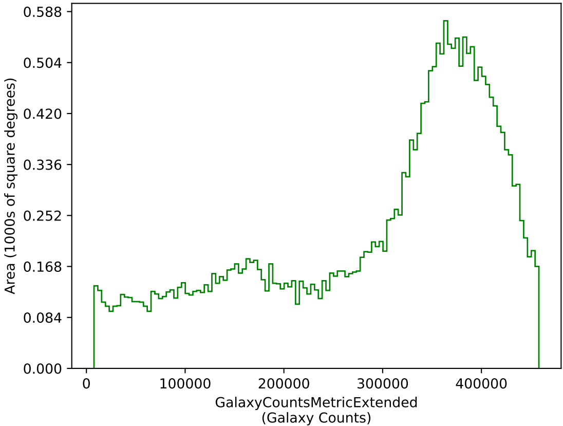
roll_mid2_const_season6v3.3_10yrs g: GalaxyCountsMetricExtended
