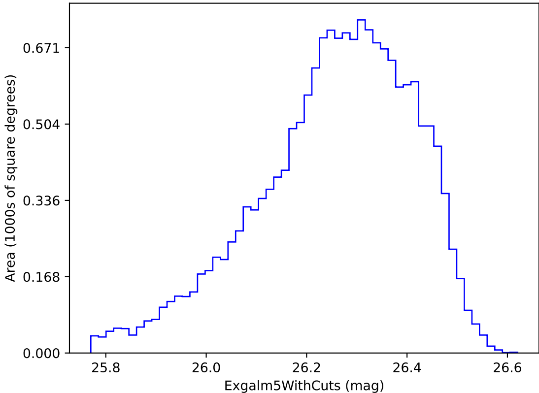
roll_mid2_const_season6v3.3_10yrs i band non-DD year 8: ExgalM5WithCuts
