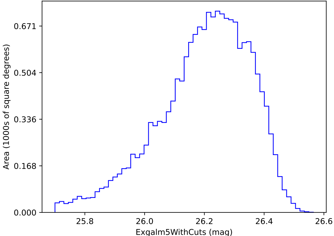
roll_mid2_const_season6v3.3_10yrs i band non-DD year 7: ExgalM5WithCuts
