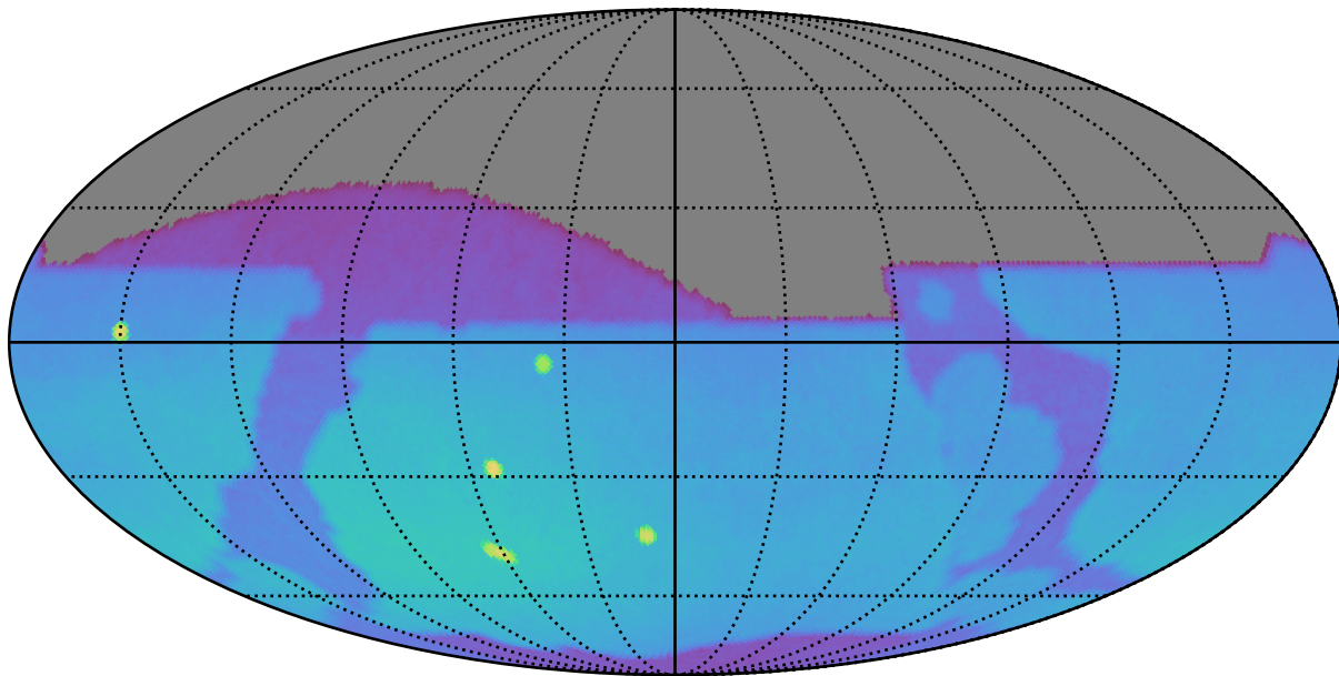
roll_mid2_const_season6v3.3_10yrs : Brown Dwarf, L4
