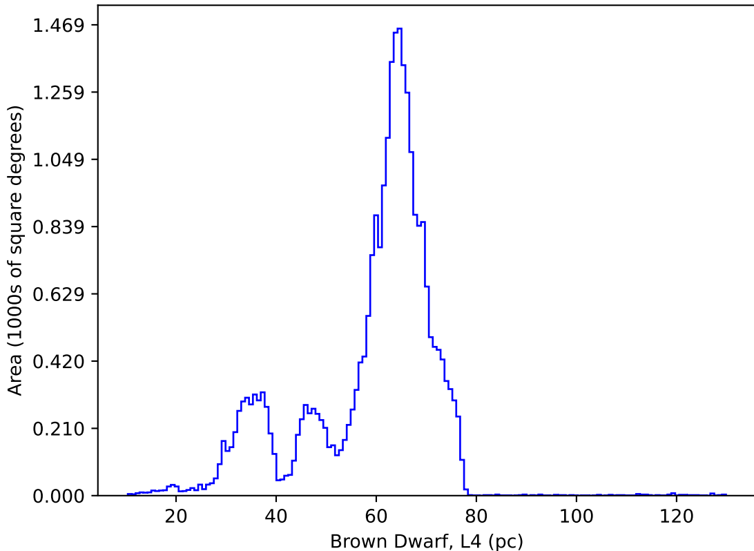
roll_mid2_const_season6v3.3_10yrs : Brown Dwarf, L4
