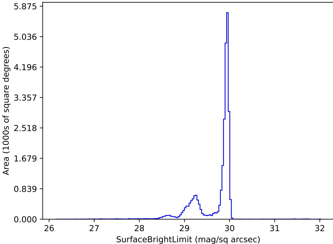
roll_mid1_const_season4v3.3_10yrs i: SurfaceBrightLimit
