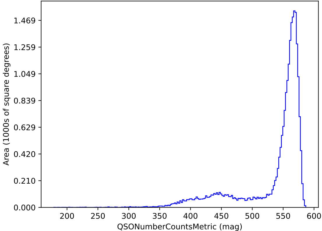
roll_mid1_const_season4v3.3_10yrs y band and non-DD: QSONumberCountsMetric
