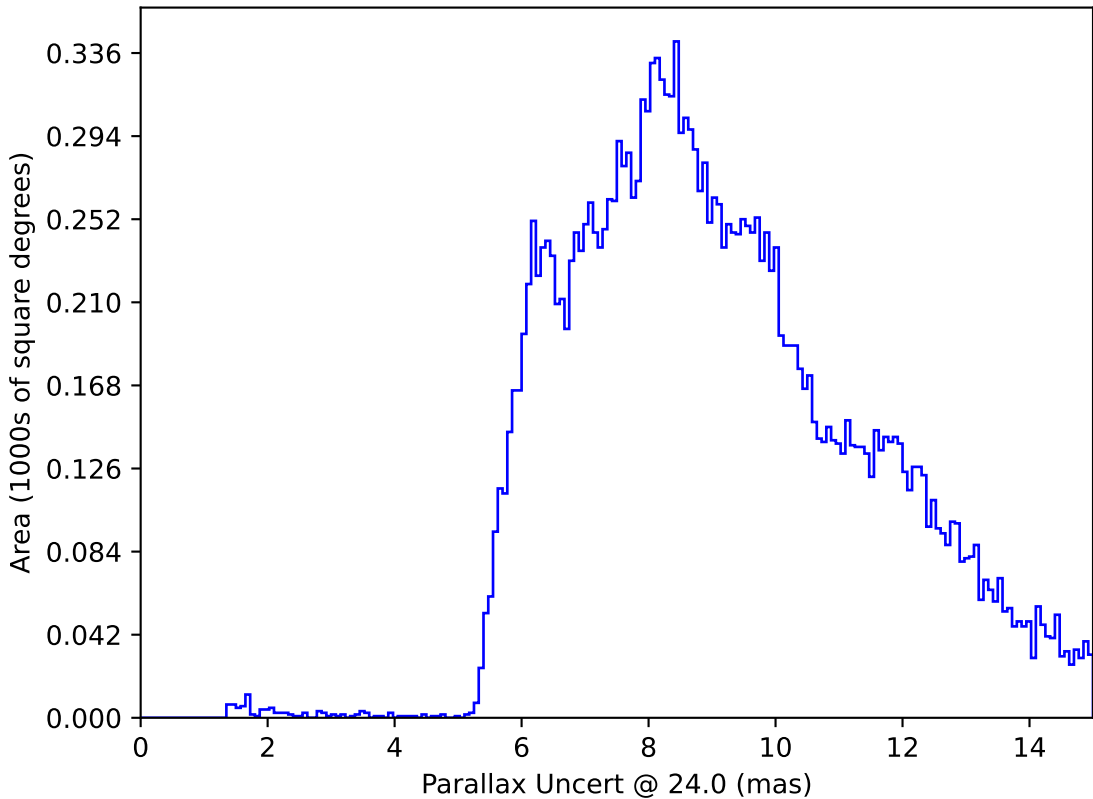
roll_mid1_const_season4v3.3_10yrs : Parallax Uncert @ 24.0
