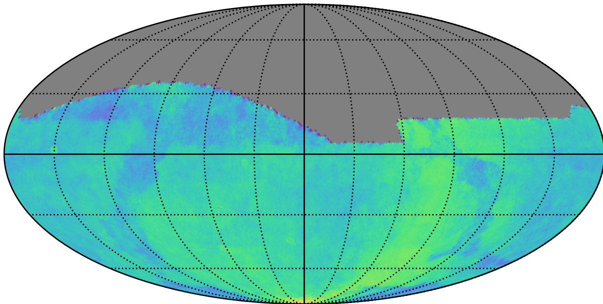
roll_mid1_const_season4v3.3_10yrs : Parallax Coverage @ 24.0
