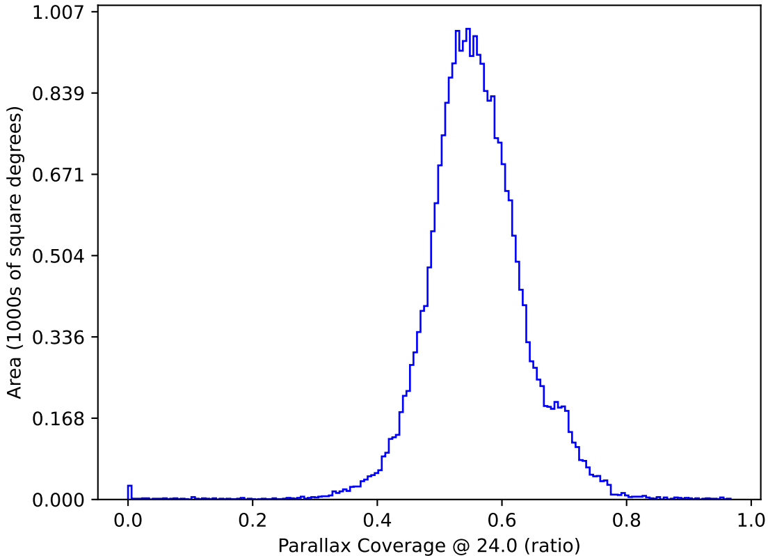
roll_mid1_const_season4v3.3_10yrs : Parallax Coverage @ 24.0
