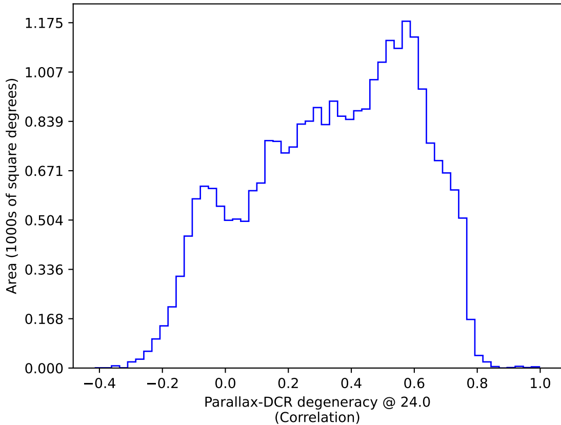
roll_mid1_const_season4v3.3_10yrs : Parallax-DCR degeneracy @ 24.0
