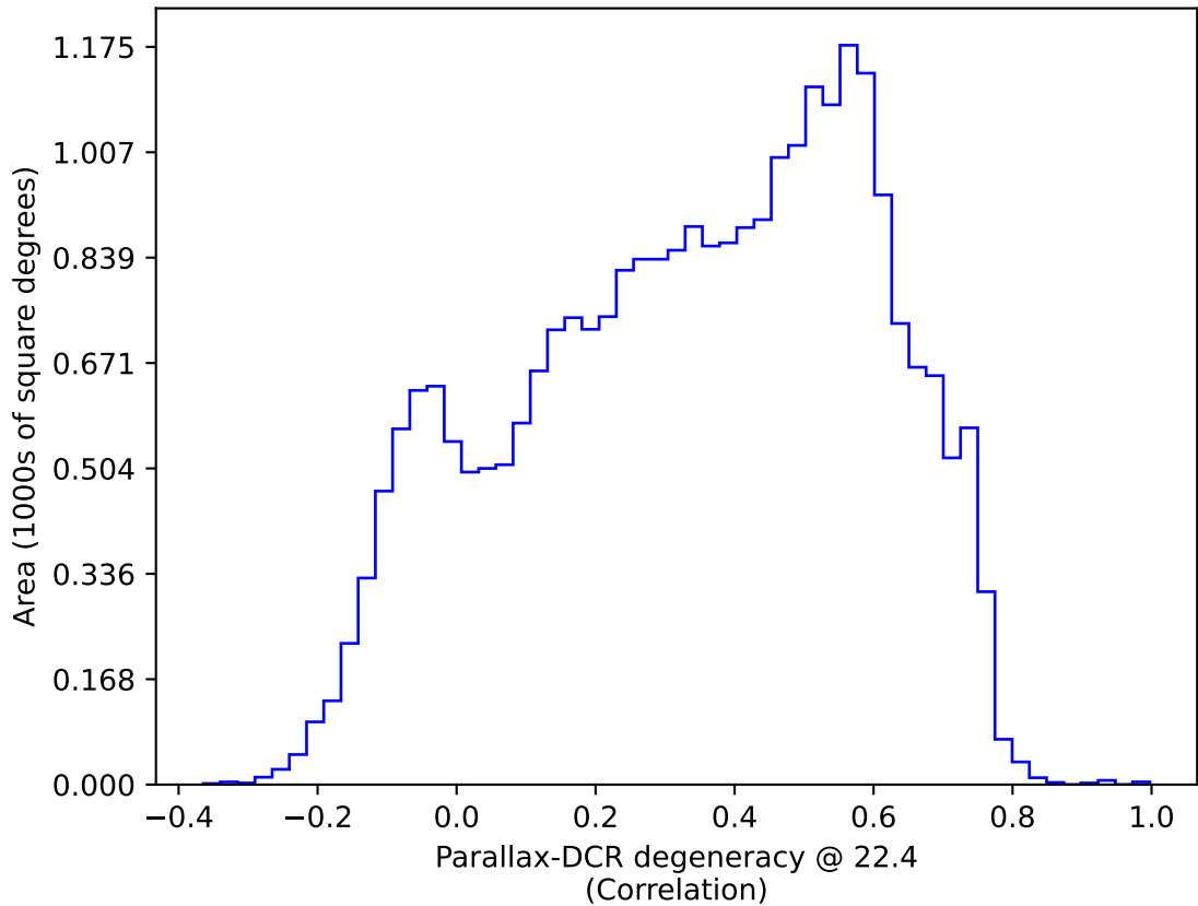
roll_mid1_const_season4v3.3_10yrs : Parallax-DCR degeneracy @ 22.4
