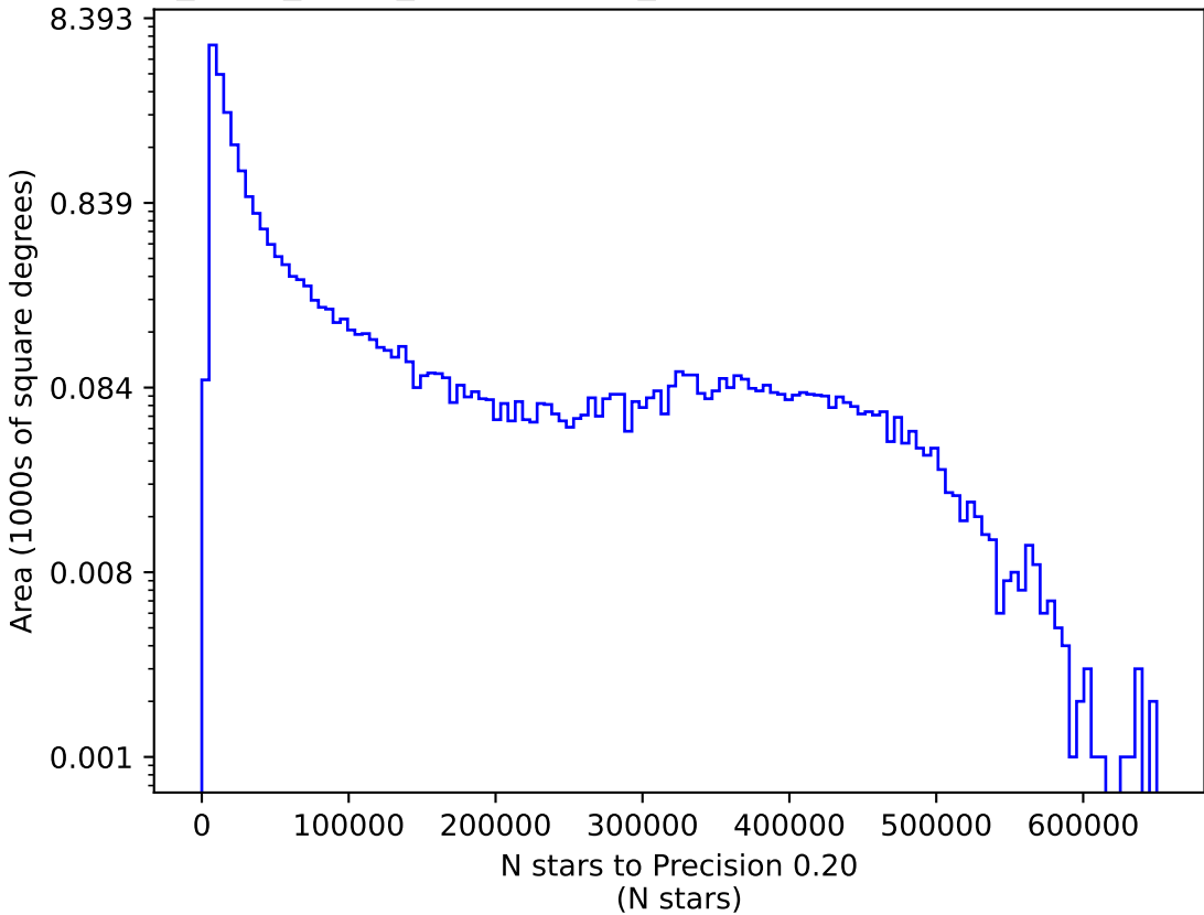
roll_mid1_const_season4v3.3_10yrs z: N stars to Precision 0.20
