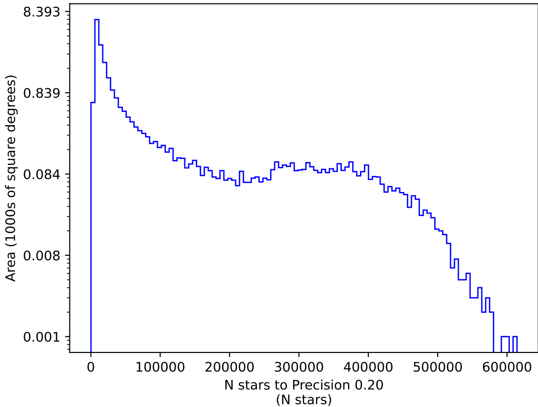
roll_mid1_const_season4v3.3_10yrs y: N stars to Precision 0.20
