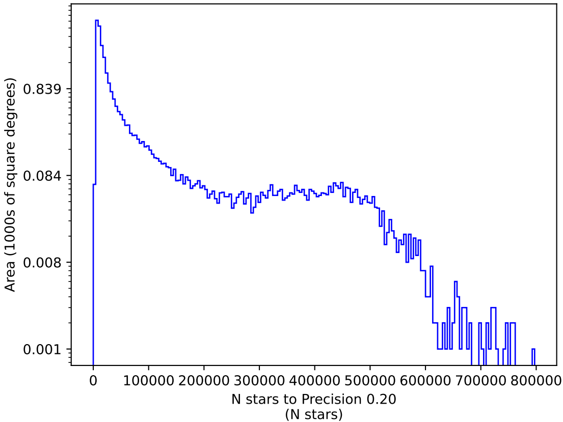
roll_mid1_const_season4v3.3_10yrs r: N stars to Precision 0.20
