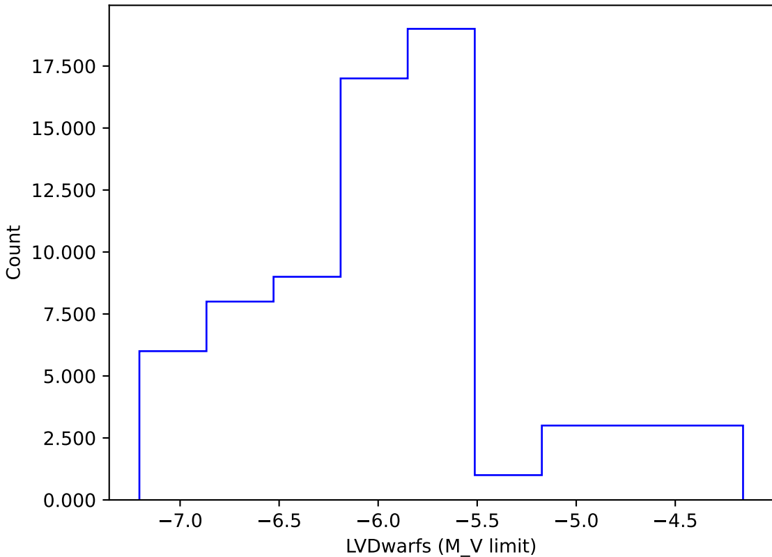
roll_mid1_const_season4v3.3_10yrs gi: LVDwarfs
