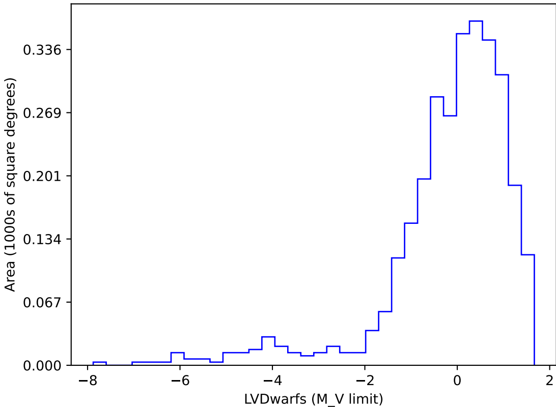
roll_mid1_const_season4v3.3_10yrs gi SCP: LVDwarfs
