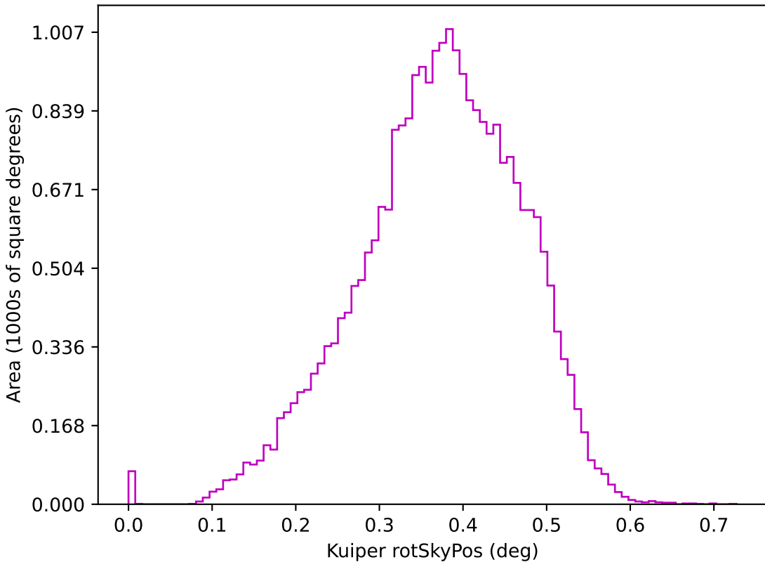
roll_mid1_const_season4v3.3_10yrs z: Kuiper rotSkyPos
