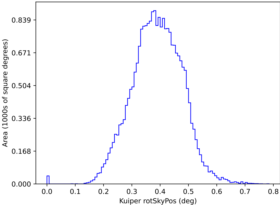
roll_mid1_const_season4v3.3_10yrs y: Kuiper rotSkyPos
