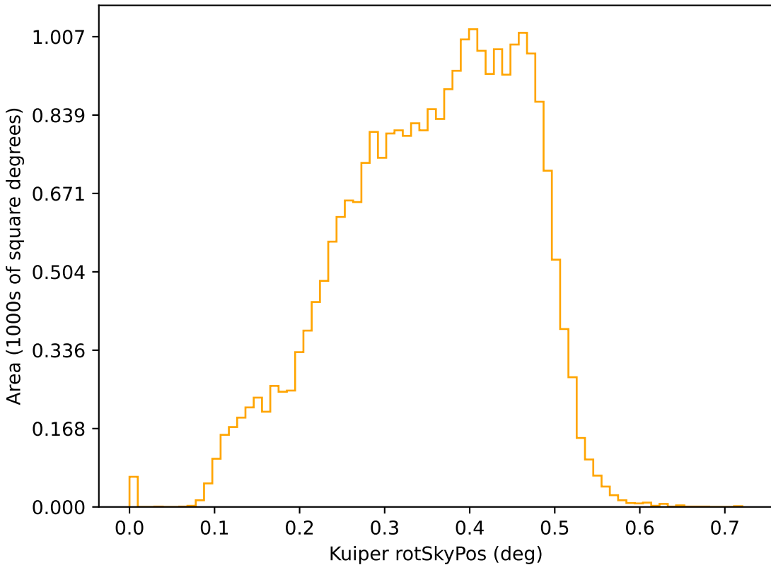
roll_mid1_const_season4v3.3_10yrs r: Kuiper rotSkyPos
