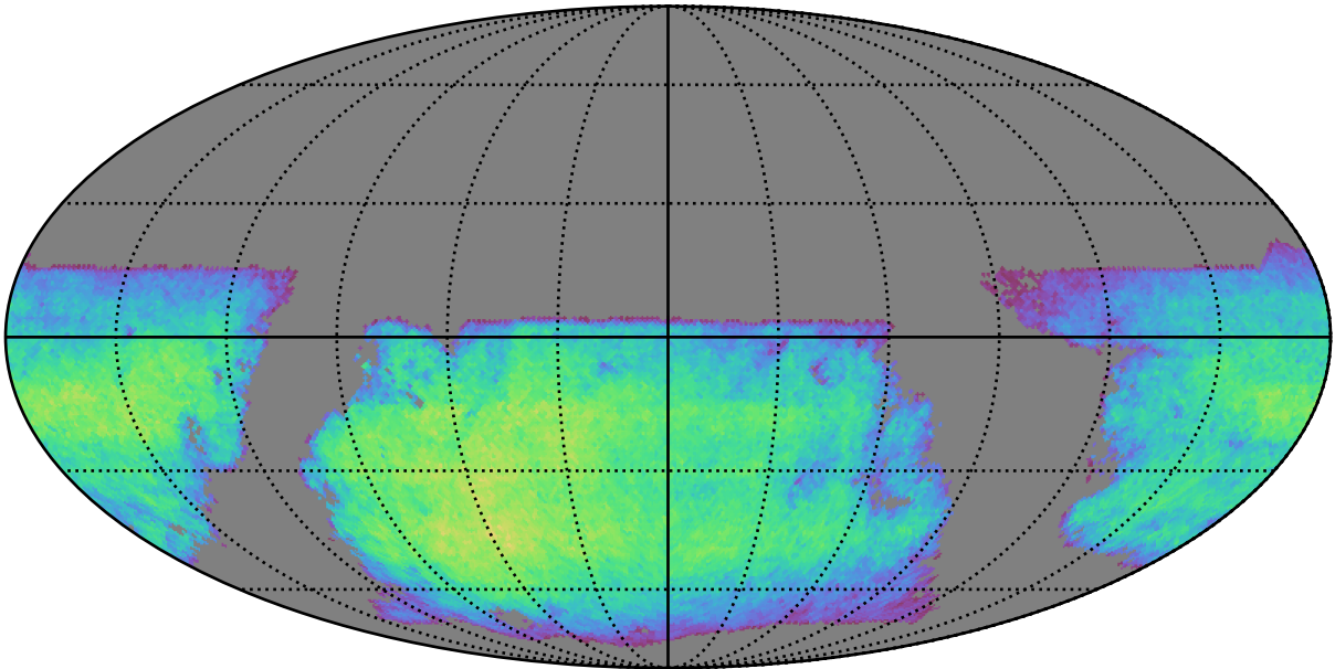
roll_mid1_const_season4v3.3_10yrs i band non-DD year 9: ExgalM5WithCuts
