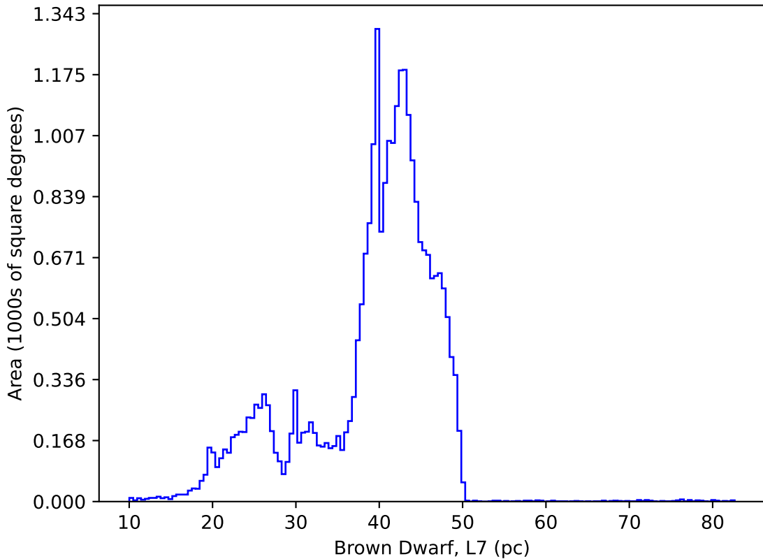
roll_mid1_const_season4v3.3_10yrs : Brown Dwarf, L7
