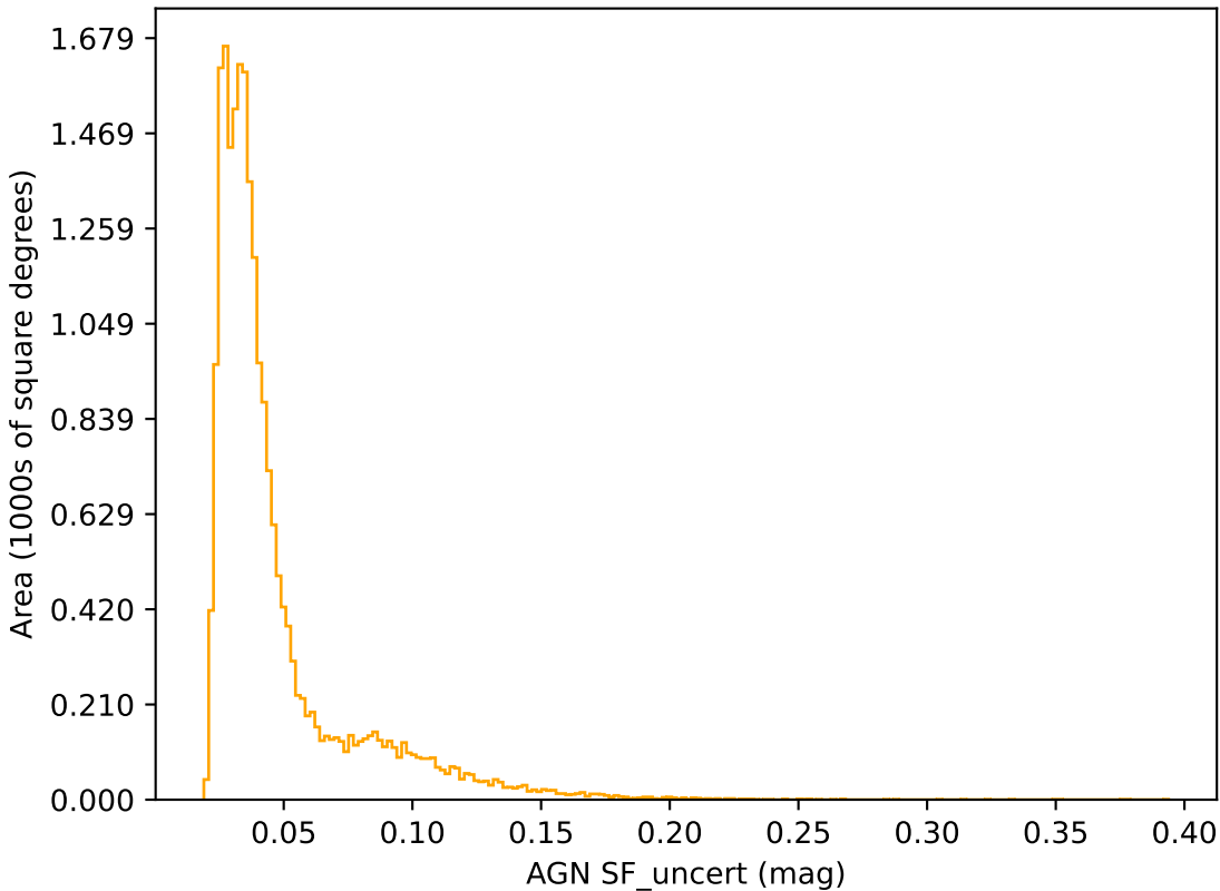
roll_mid1_const_season4v3.3_10yrs r band: AGN SF_uncert
