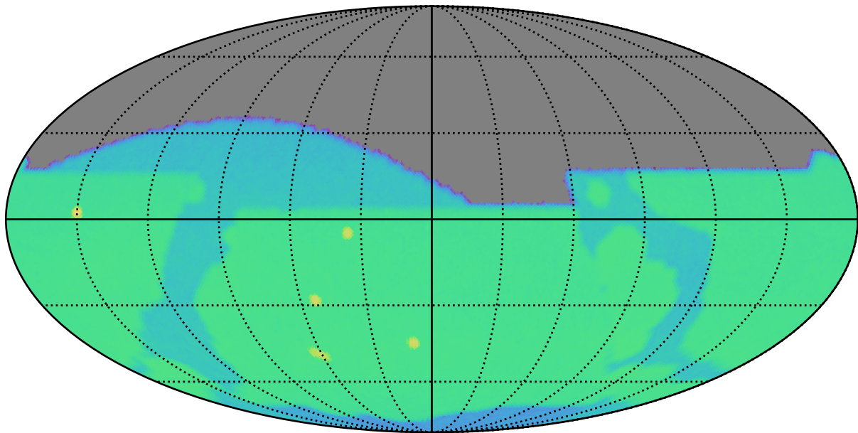
roll_mid1_const_season2v3.3_10yrs r: SurfaceBrightLimit
