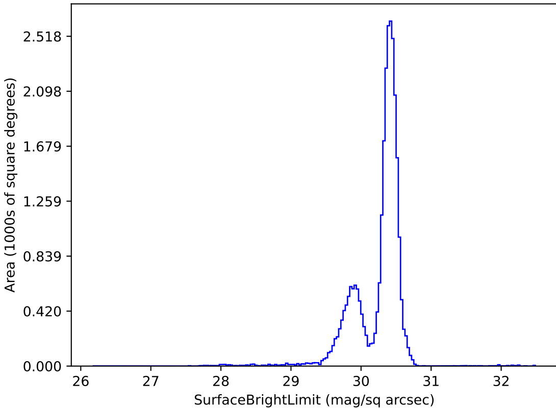
roll_mid1_const_season2v3.3_10yrs g: SurfaceBrightLimit
