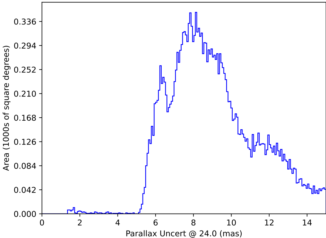
roll_mid1_const_season2v3.3_10yrs : Parallax Uncert @ 24.0
