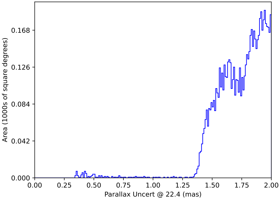
roll_mid1_const_season2v3.3_10yrs : Parallax Uncert @ 22.4
