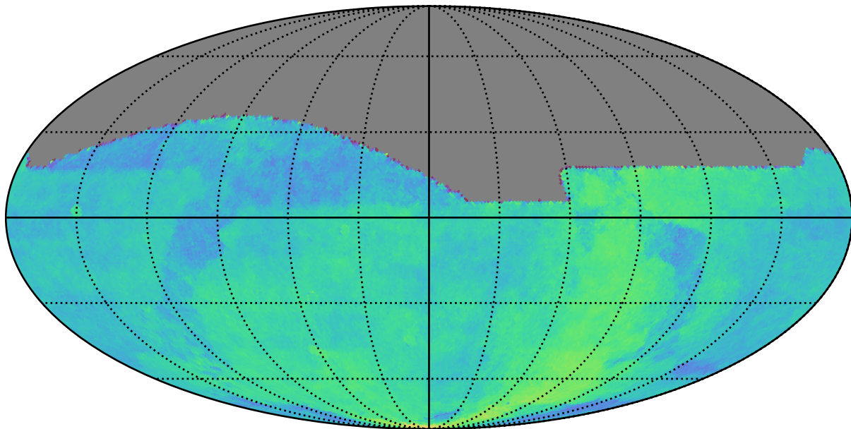
roll_mid1_const_season2v3.3_10yrs : Parallax Coverage @ 24.0
