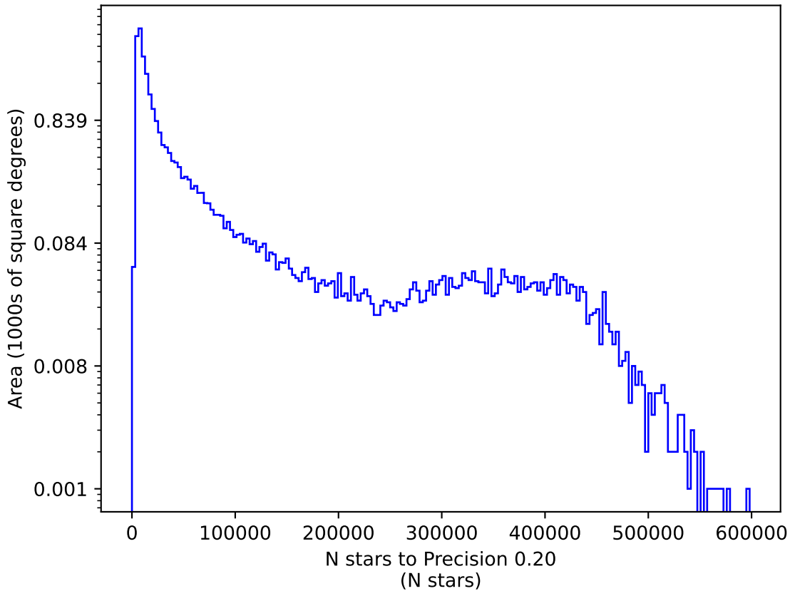
roll_mid1_const_season2v3.3_10yrs g: N stars to Precision 0.20
