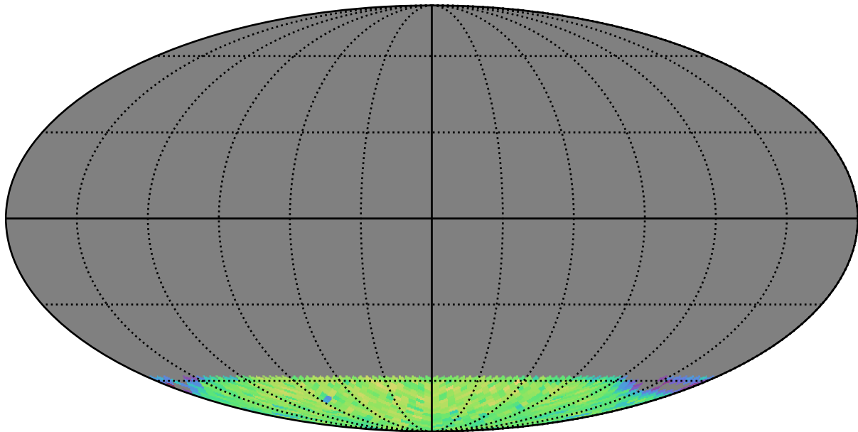
roll_mid1_const_season2v3.3_10yrs gi SCP: LVDwarfs
