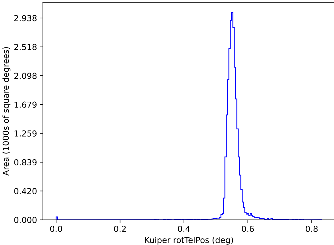
roll_mid1_const_season2v3.3_10yrs y: Kuiper rotTelPos
