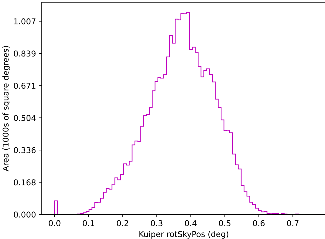
roll_mid1_const_season2v3.3_10yrs z: Kuiper rotSkyPos
