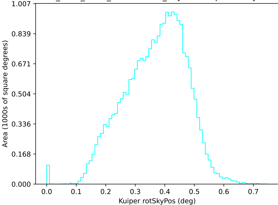
roll_mid1_const_season2v3.3_10yrs u: Kuiper rotSkyPos
