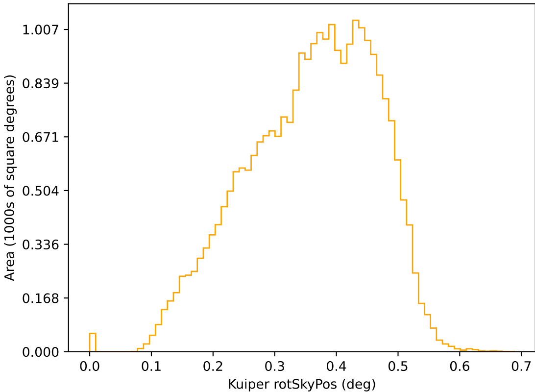
roll_mid1_const_season2v3.3_10yrs r: Kuiper rotSkyPos
