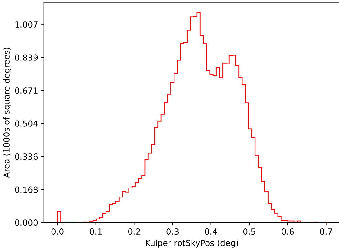
roll_mid1_const_season2v3.3_10yrs i: Kuiper rotSkyPos
